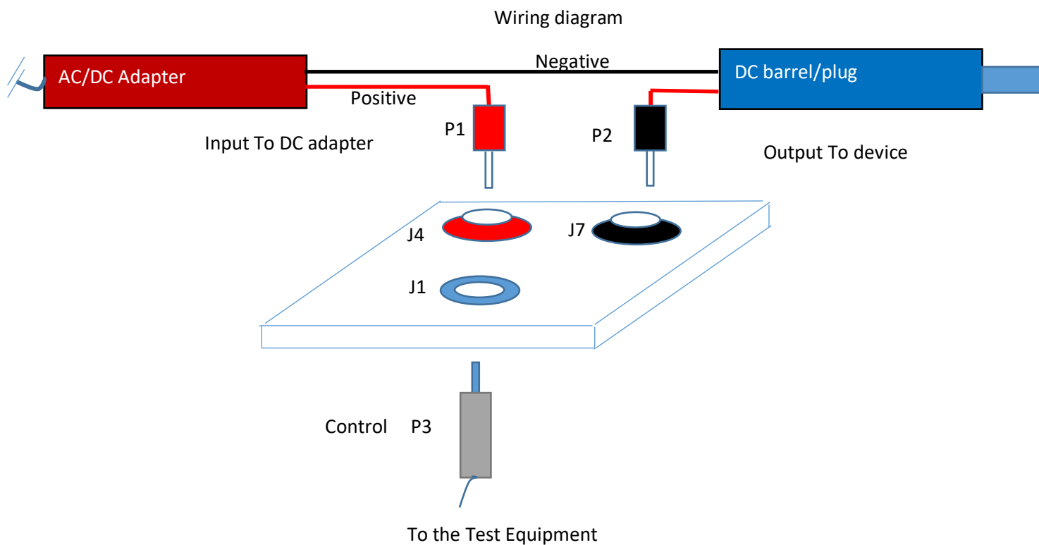
Figure 9 Wiring diagram
